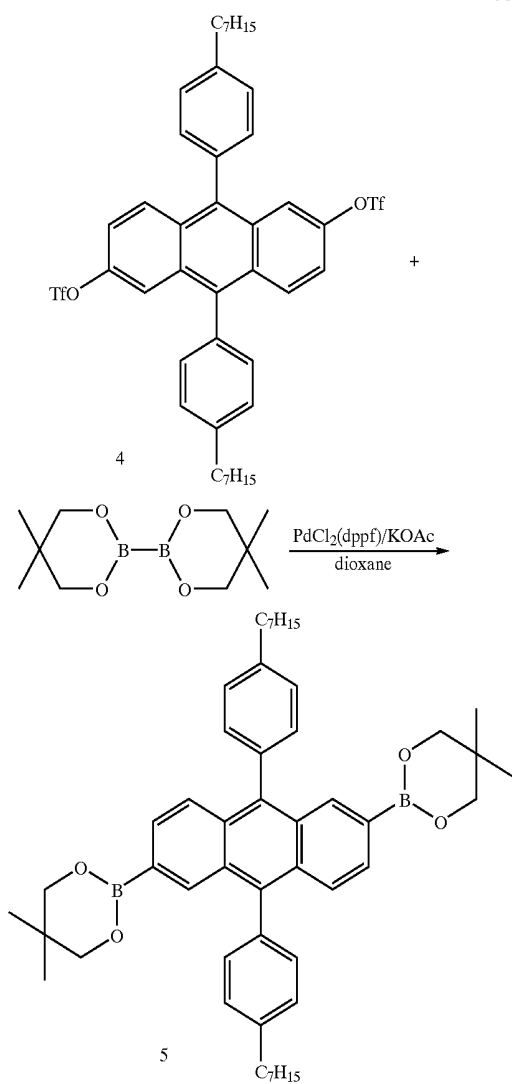
Scheme 2
