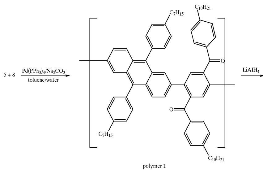
Scheme 3 Synthesis of Polymers
